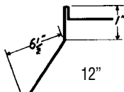
Gravel Stop for Shingle
